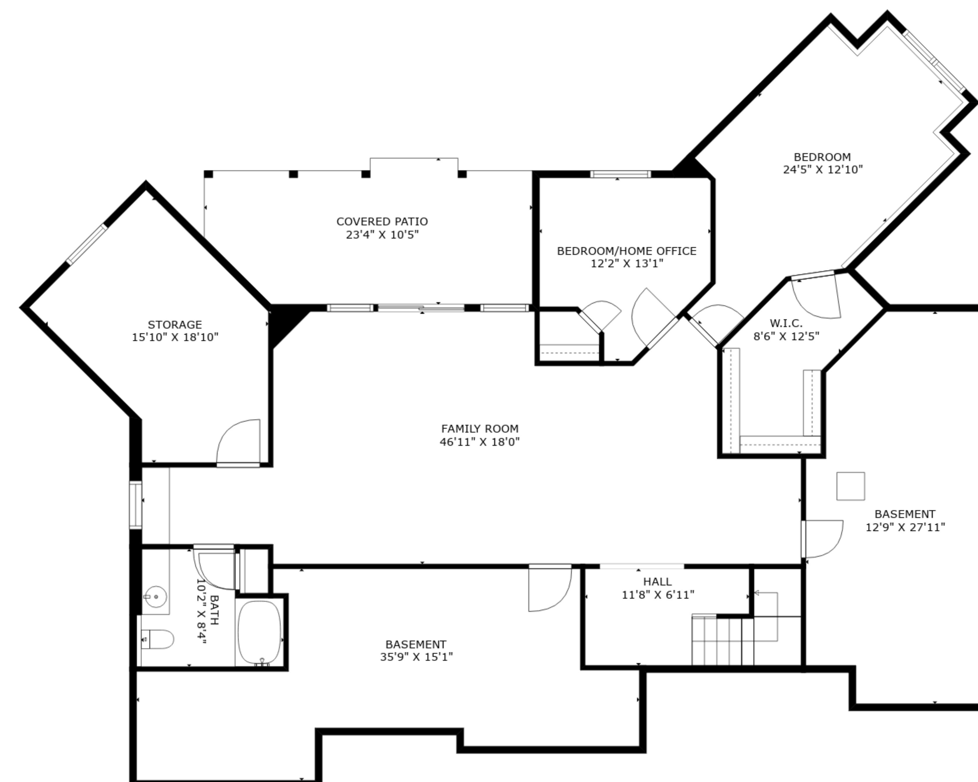
FLOOR 1
